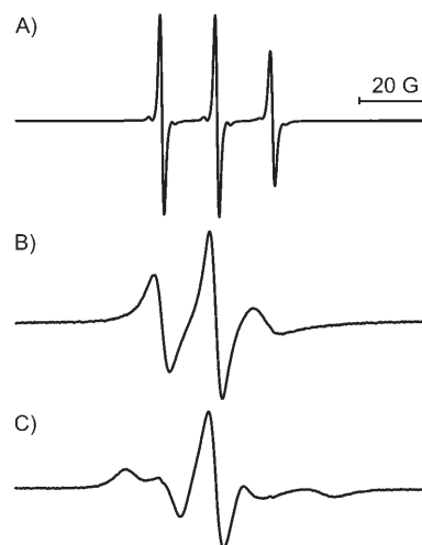
Figure 2. EPR spectra, recorded in aqueous solution (10 mM phosphate buffer, pH 7.0, 100 mM NaCl, 0.1 mM EDTA) at 20°C: A) spin-labeled nucleoside 9 ; B) spin-labeled oligomer 5'-d(GACCTCG- \dot{\text{C}} ATCGTG); and C) spin-labeled duplex 5'-d(GACCTCG \dot{\text{C}} ATCGTG)·5'-d(CACGATGCGAGGTC).
